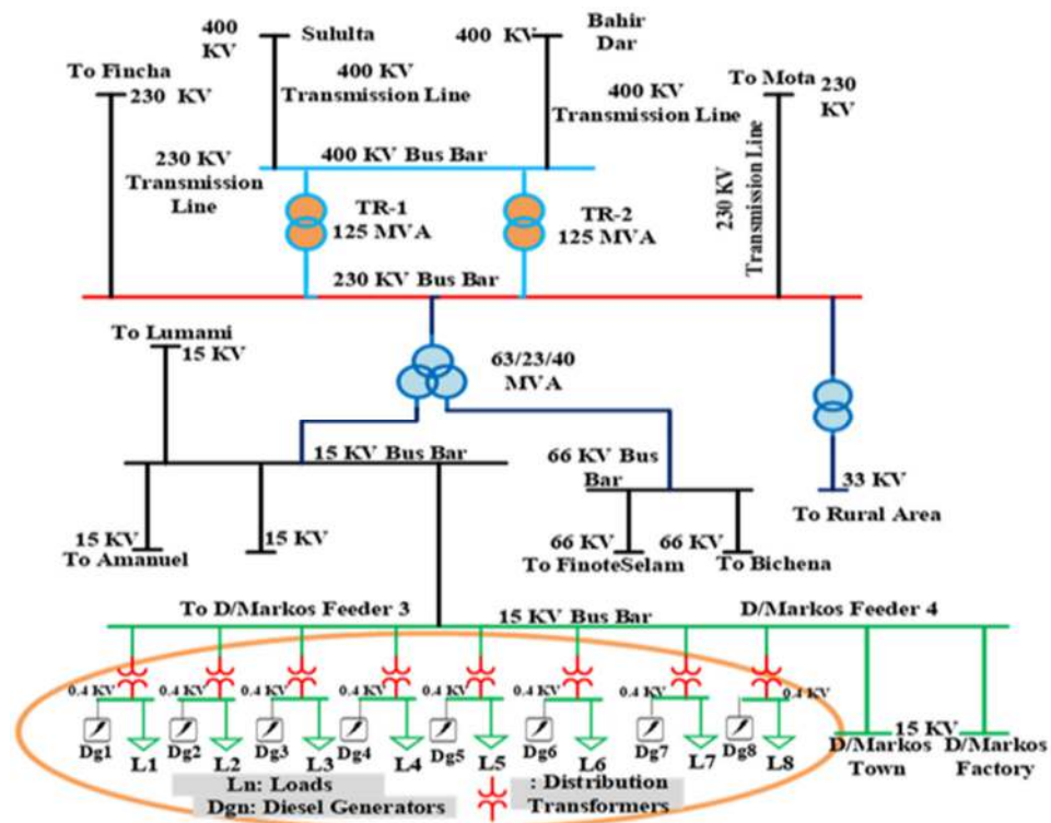
Figure 3. Existing distribution network schematic diagram on the study area.
