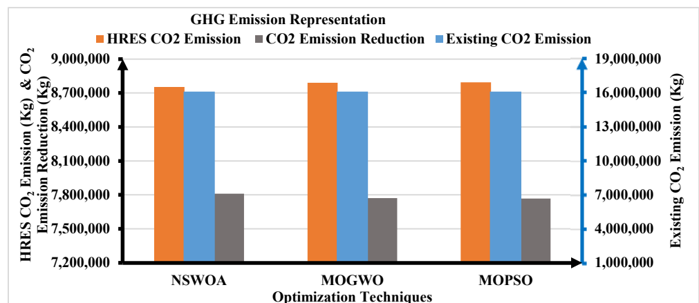
Figure 10. GHG emissions parameters [ CO_2Emissions , P_{HRES} and P_{EA} ] representations using NSWOA, MOGWO, and MOPSO techniques.
