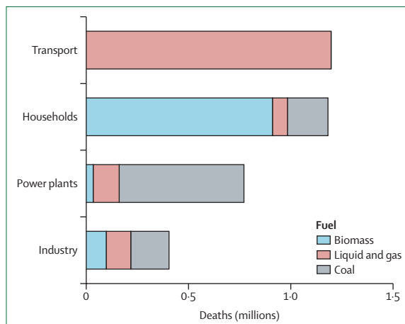
Figure 2: Estimated deaths from PM 2.5 exposure, by fuel and sector in 2022 Liquid gas includes light and heavy oil, diesel oil, and natural gas. Coal includes hard and brown coals and coal coke. Biomass includes wood, charcoal, dung, and agricultural residue. Data are from The Lancet's 2025 Countdown on health and climate change indicator modelling premature mortality from air pollution. The model estimates concentrations and exposures by use of emissions inventories and chemical dispersion models and estimates health impacts by use of PM 2.5 exposure–response relationships. 35
